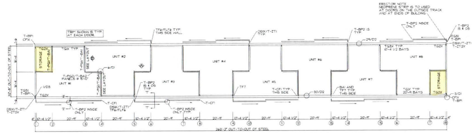
PARTITION & TRACK LAYOUT
