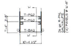
PARTITION ELEVATION "A" (9 PLACES)
