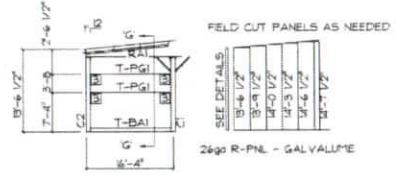
PARTITION ELEVATION "B" (6 PLACES)
