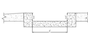
CONCRETE MEDIAN SW
