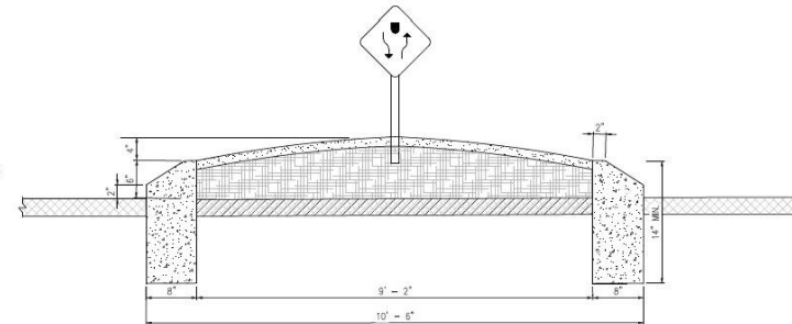
GRASSED MEDIAN DETAIL
