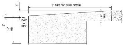
TYPE "N" SPECIAL CURB
