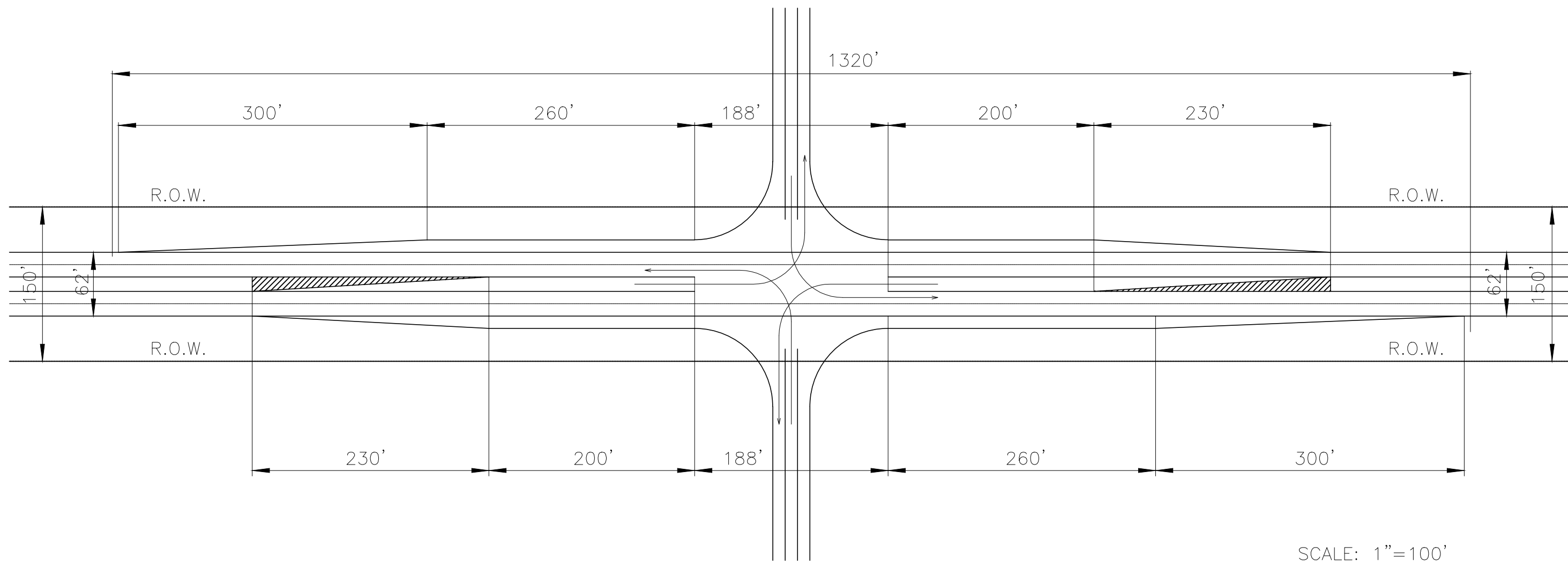
FOLEY — BEACH EXPRESS TYPICAL DUAL CROSS-OVER ACCESS UNIT FOR 150' RIGHT OF WAY EXHIBIT C-1
