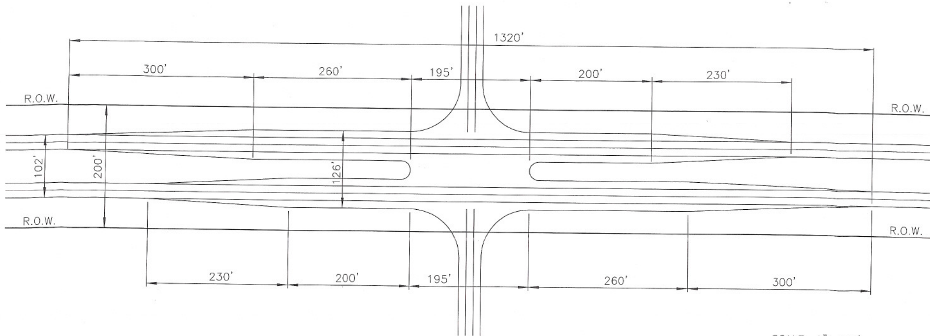
FOLEY - BEACH EXPRESS TYPICAL DUAL CROSS-OVER ACCESS UNIT FOR 200' RIGHT OF WAY EXHIBIT E (200')
