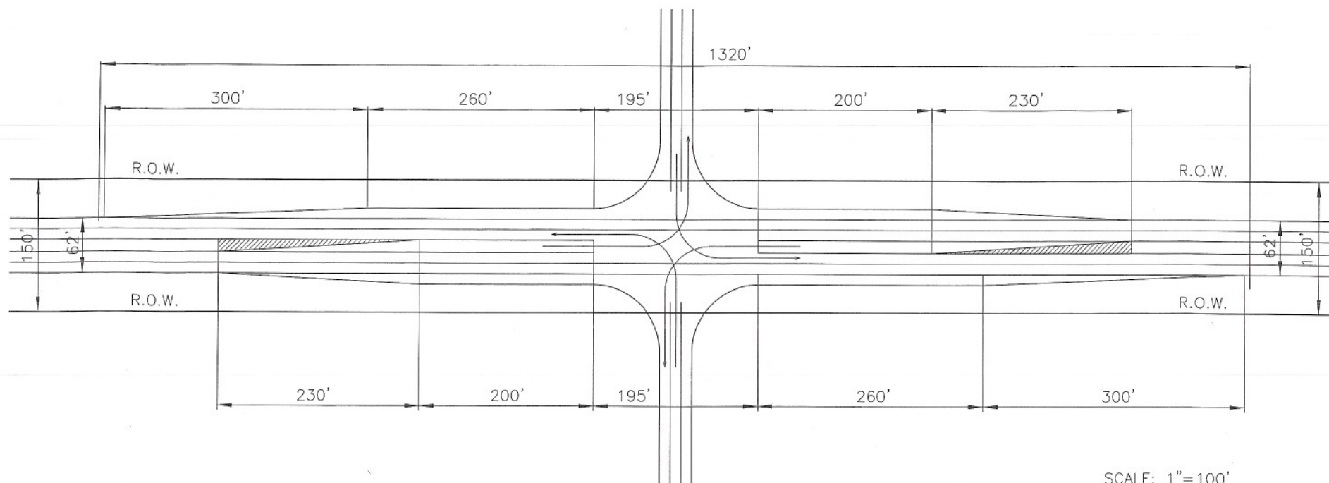
FOLEY — BEACH EXPRESS TYPICAL DUAL CROSS-OVER ACCESS UNIT FOR 150' RIGHT OF WAY EXHIBIT G E (150')
