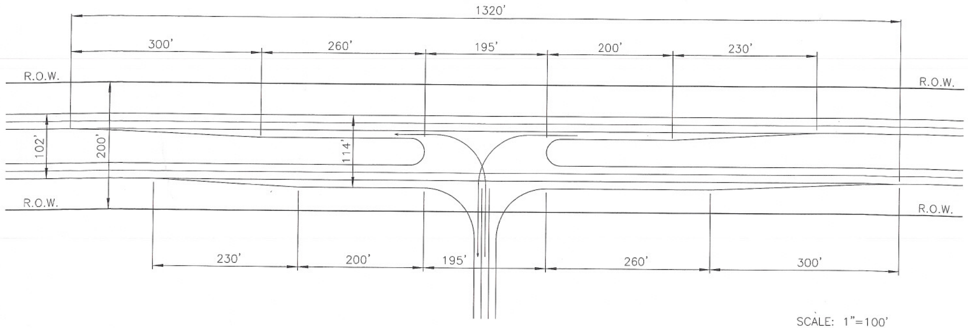
FOLEY — BEACH EXPRESS TYPICAL CROSS-OVER ACCESS UNIT FOR 200' RIGHT OF WAY EXHIBIT D (200')
